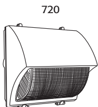
720 Height 12.0" Width 11.125" Depth 7.875"
